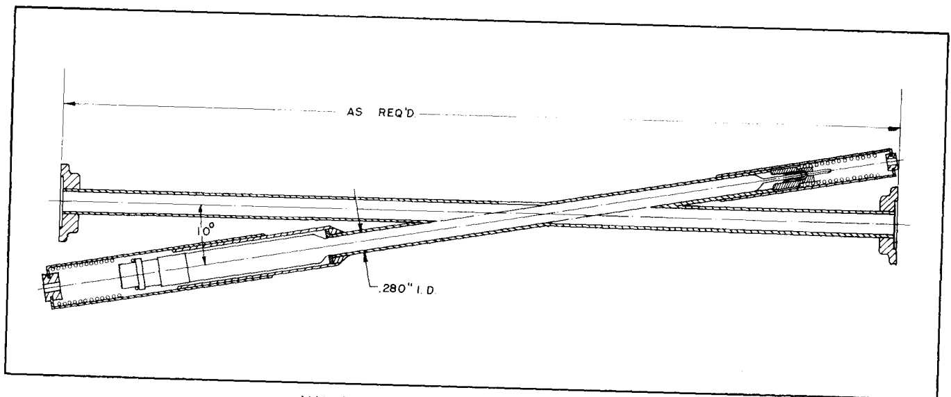
WAVEGUIDE MOUNT ASSEMBLY RG-91/U
