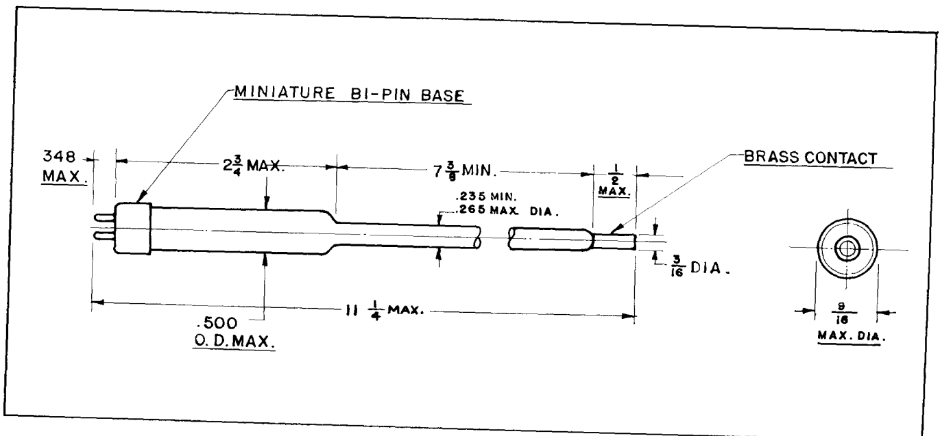
OUTLINE DRAWING
