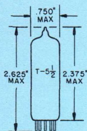
GLASS BULB
