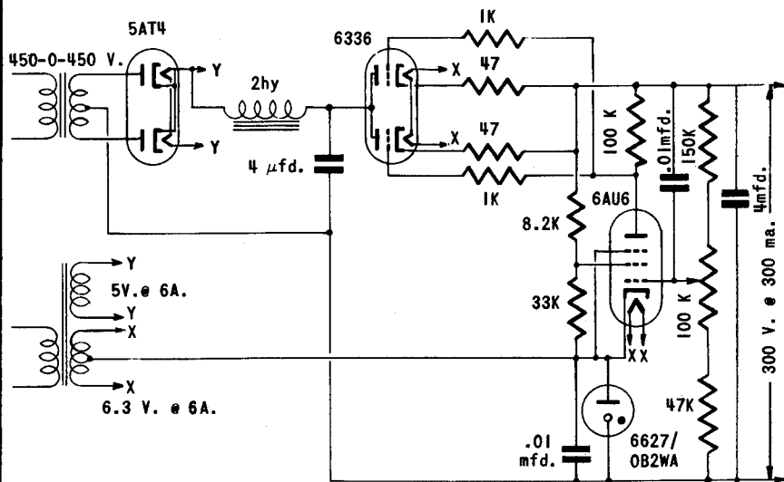
TYPICAL APPLICATION OF 6627/0B2WA USED IN VOLTAGE REGULATED POWER SUPPLY FIGURE 4
