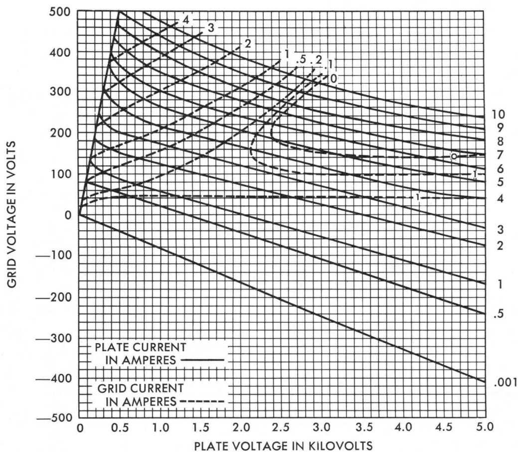
CONSTANT CURRENT CHARACTERISTICS
