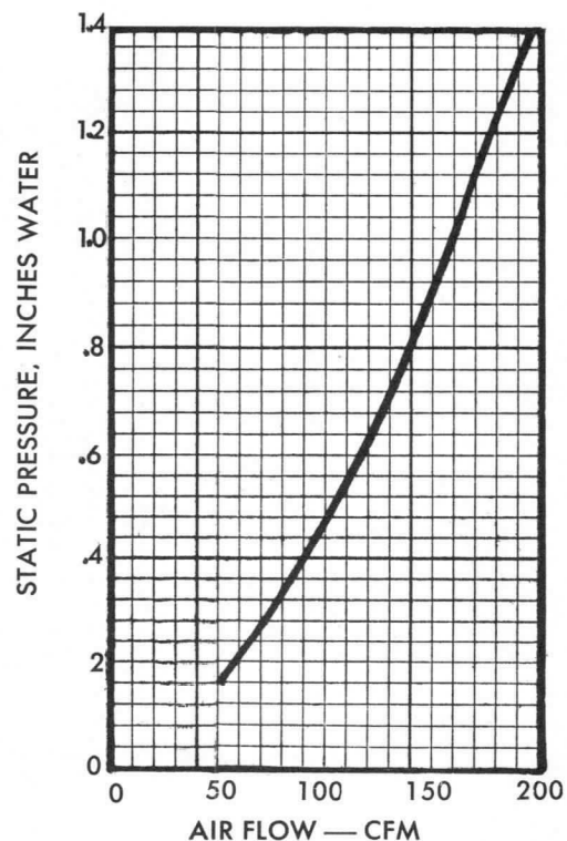
AIR COOLING CHARACTERISTICS
