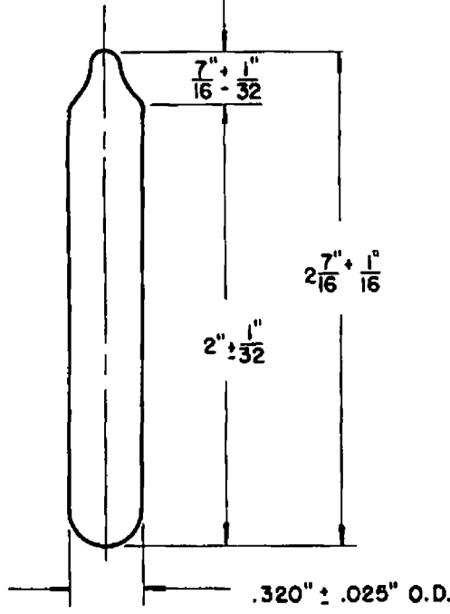
K-69087-186A78 OUTLINE GL-6620 1-24-55
