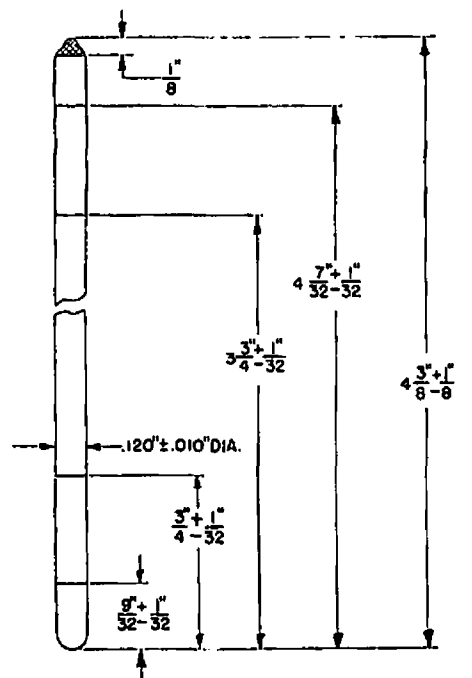
K-69087-186A67 OUTLINE GL-6619, GL-6621 1-24-55
