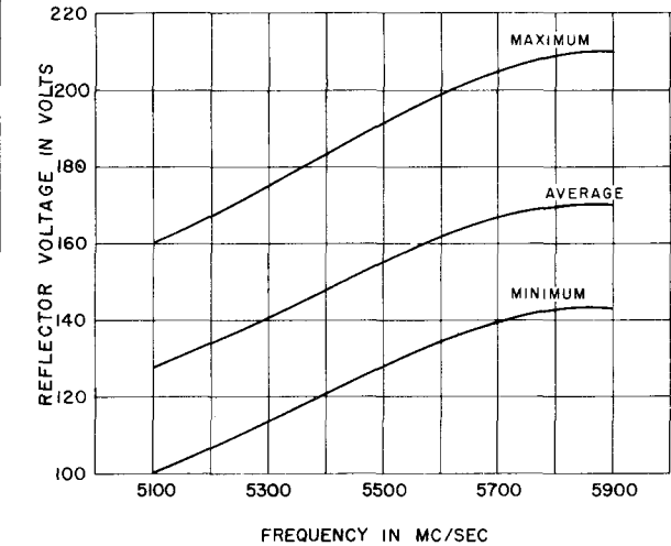
TYPICAL VARIATION OF REPELLER VOLTAGE WITH FREQUENCY
