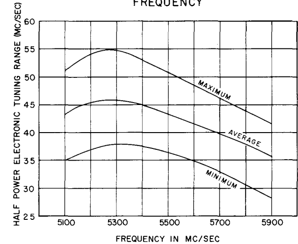
TYPICAL VARIATION OF HALF POWER ELECTRONIC TUNING RANGE WITH FREQUENCY
