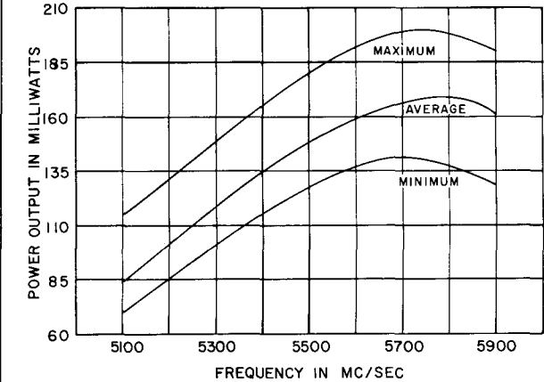
TYPICAL POWER OUTPUT VS FREQUENCY (REPELLER VOLTAGE OPTIMIZED FOR EACH FREQUENCY)
