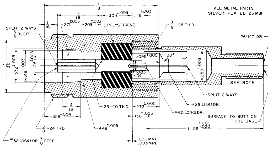
COAXIAL OUTPUT ADAPTOR
