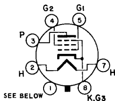
BOTTOM VIEW BASING DIAGRAM JEDEC 7AC PIN 1 - NO CONNECTION OR BASE SHELL
