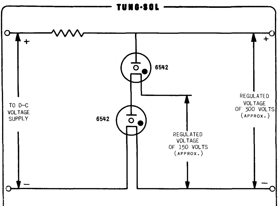
OPERATION OF REGULATOR TUBES IN SERIES FIGURE 2
