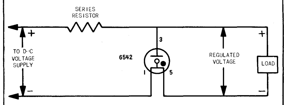
TYPICAL CIRCUIT FOR VOLTAGE REGULATOR FIGURE 3
