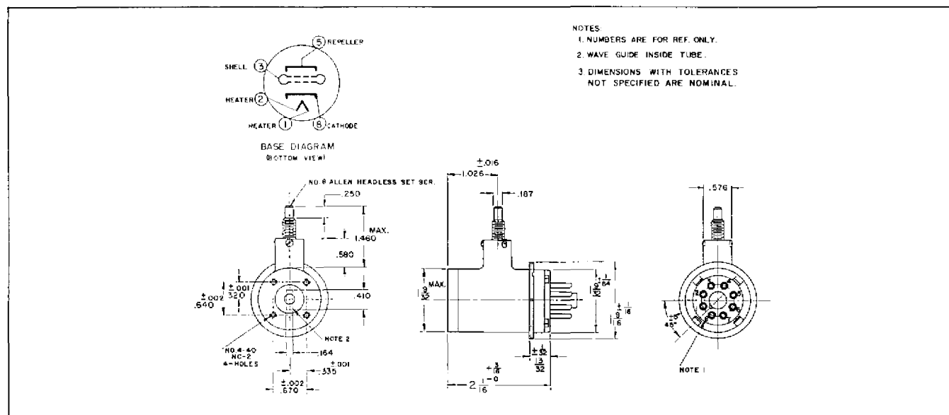
OUTLINE DRAWING
