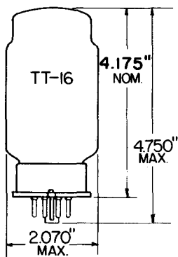
GLASS BULB
