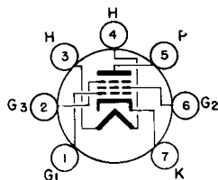
BOTTOM VIEW BASING DIAGRAM JEDEC 7CC
