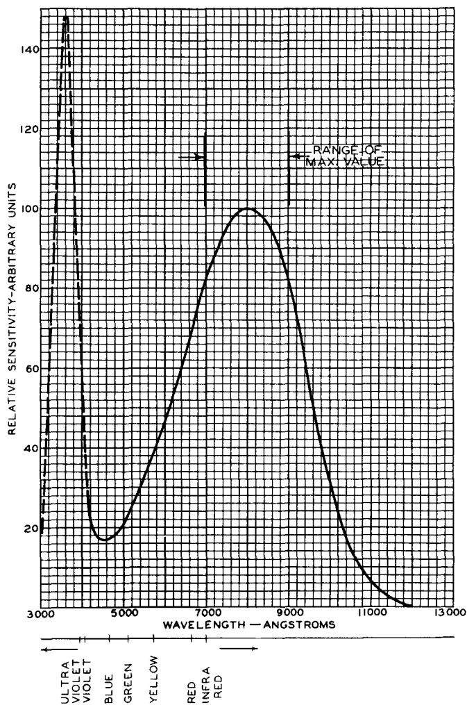
Spectral Sensitivity Characteristic of Phototube Having S-1 Response. Curve is Shown for Equal Values of Radiant Flux at All Wavelengths.
