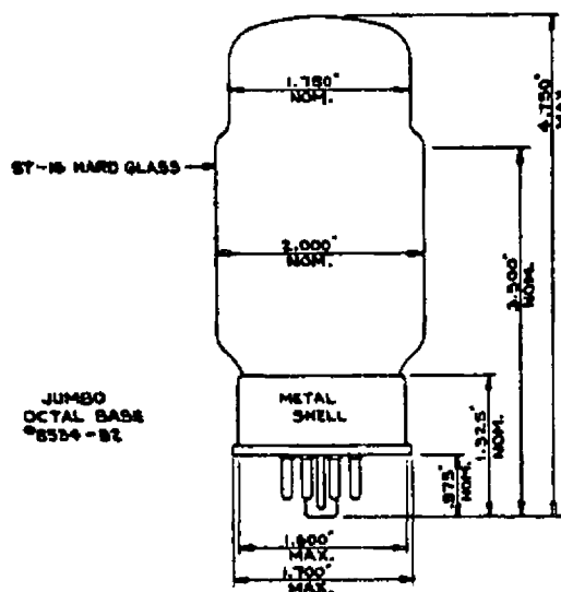
TUBE TYPE 6336-6394
