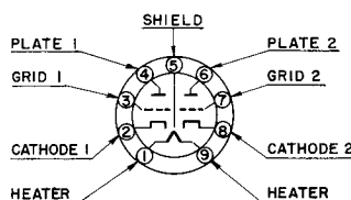
BASE DIAGRAM (BOTTOM VIEW)
