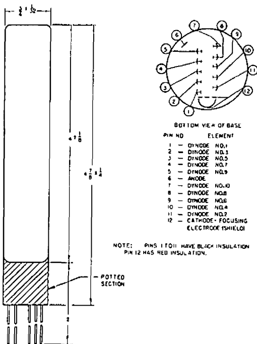
OUTLINE DRAWING TYPE 6362
