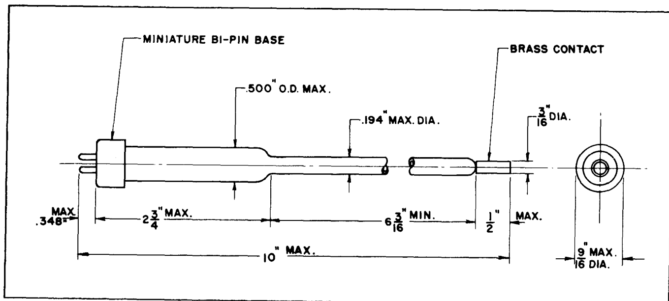
OUTLINE DRAWING
