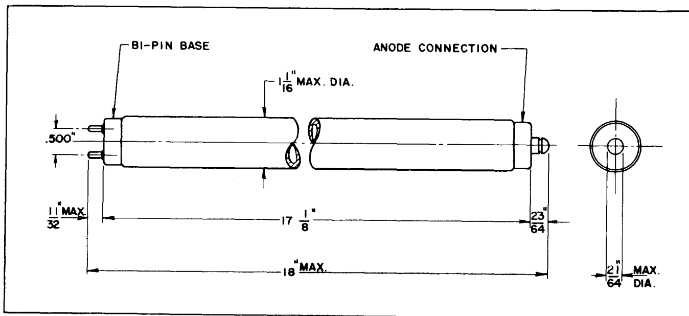
OUTLINE DRAWING
