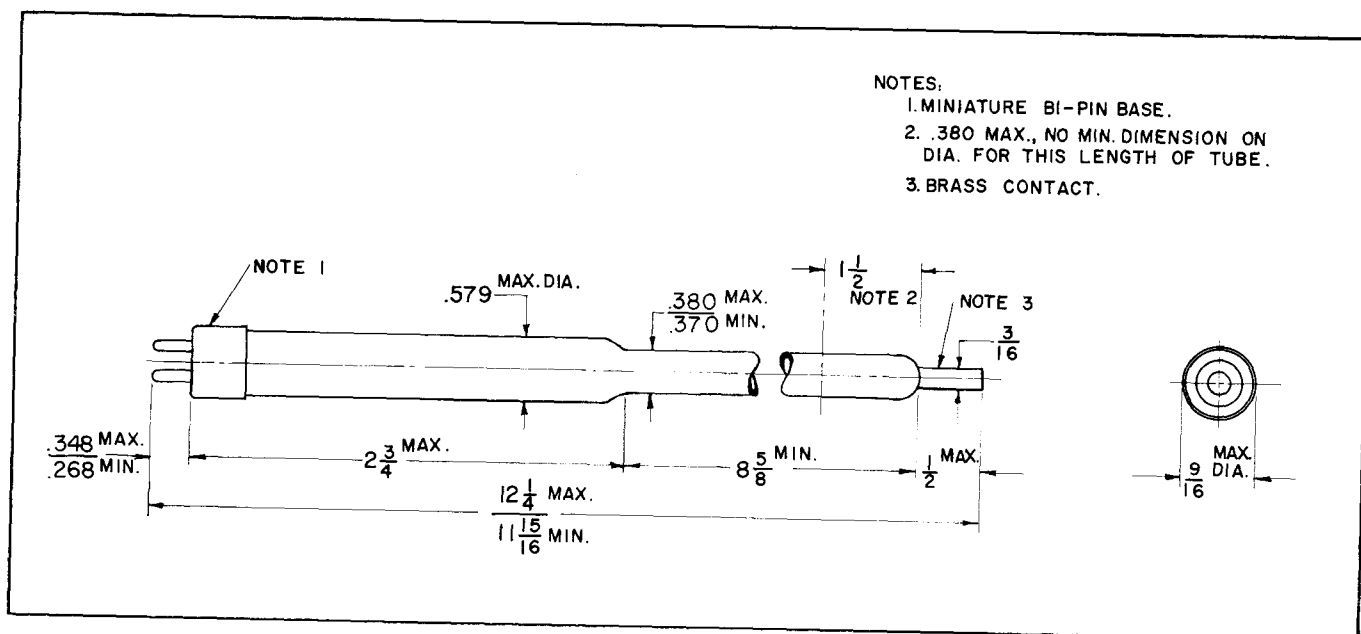
OUTLINE DRAWING
