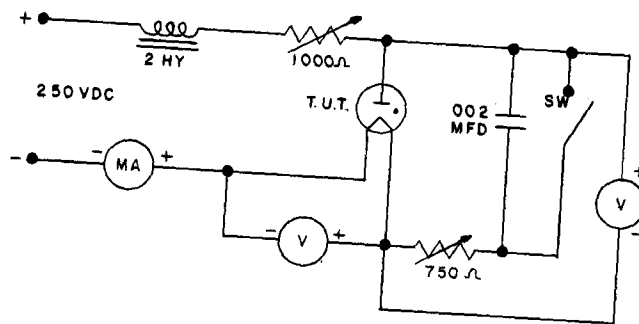
D.C. TEST CIRCUIT
