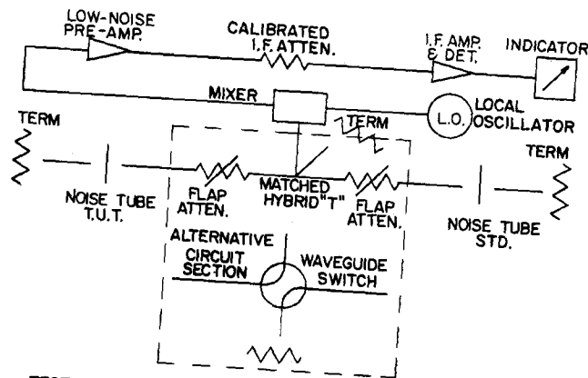
TEST CIRCUIT FOR EXCESS NOISE MEASUREMENTS
