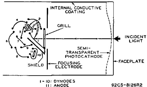
Fig. 1 - Schematic Arrangement of Type 6342-A Structure.
