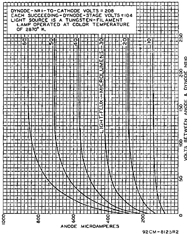
Fig. 4 - Average Anode Characteristics of Type 6342-A.
