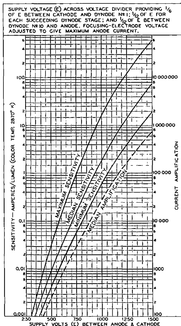
Fig. 3 - Characteristics of Type 6342-A.
