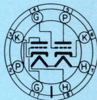
BOTTOM VIEW LARGE WAFER WITH METAL SLEEVE 8 PIN BASE
