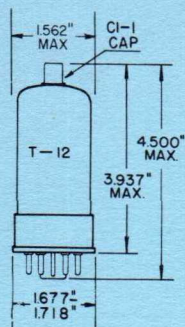
GLASS BULB LARGE WAFER MICANOL 8 PIN OCTAL WITH EXTERNAL BARRIERS AND SLEEVE BASE 88-98
