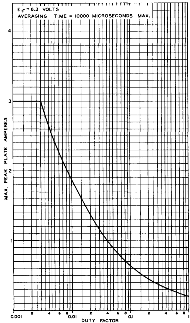
Fig. 2 - Rating Chart II for Type 6293.
