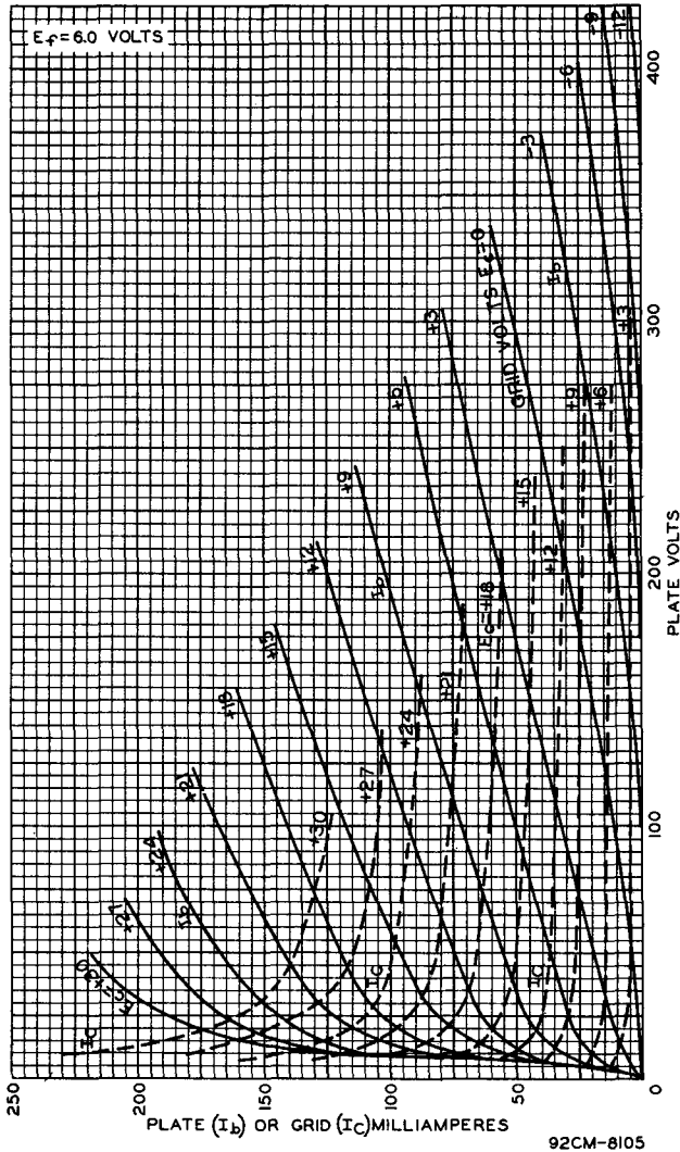
Fig. 2 - Average Plate Characteristics of Type 6264.
