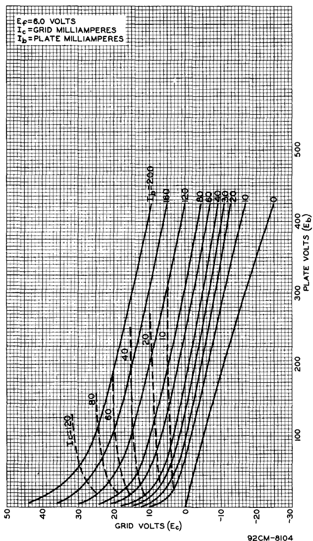
Fig. 3 - Average Constant-Current Characteristics for Type 6263.
