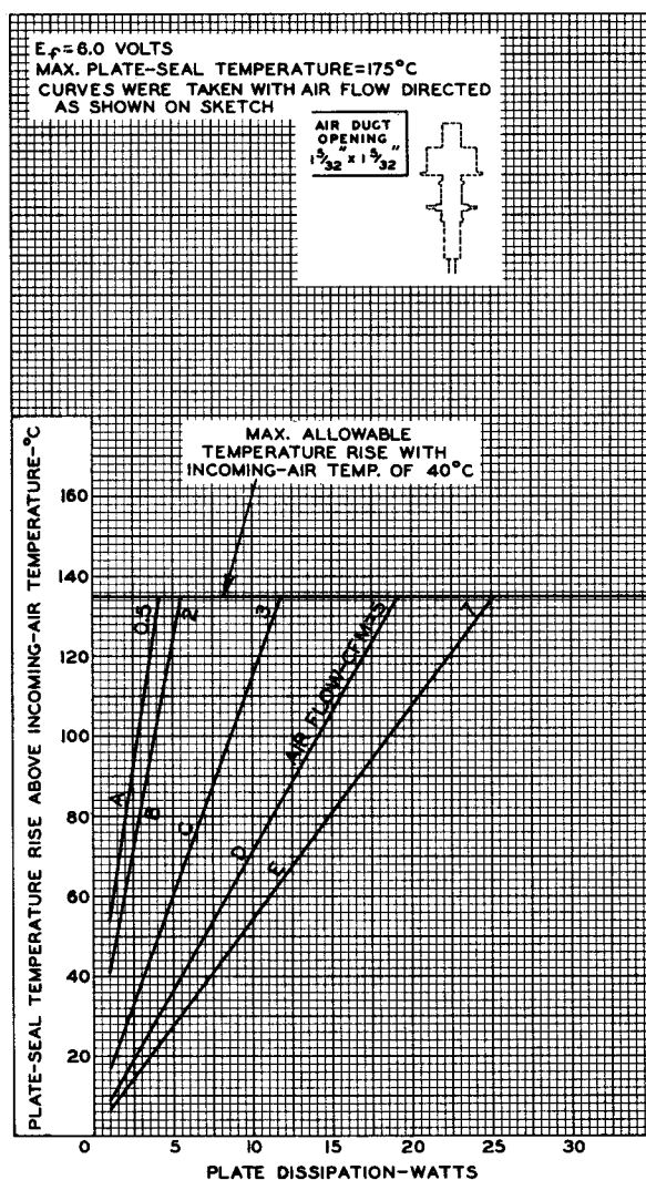
Fig. 1 - Cooling Requirements for Type 6263.
