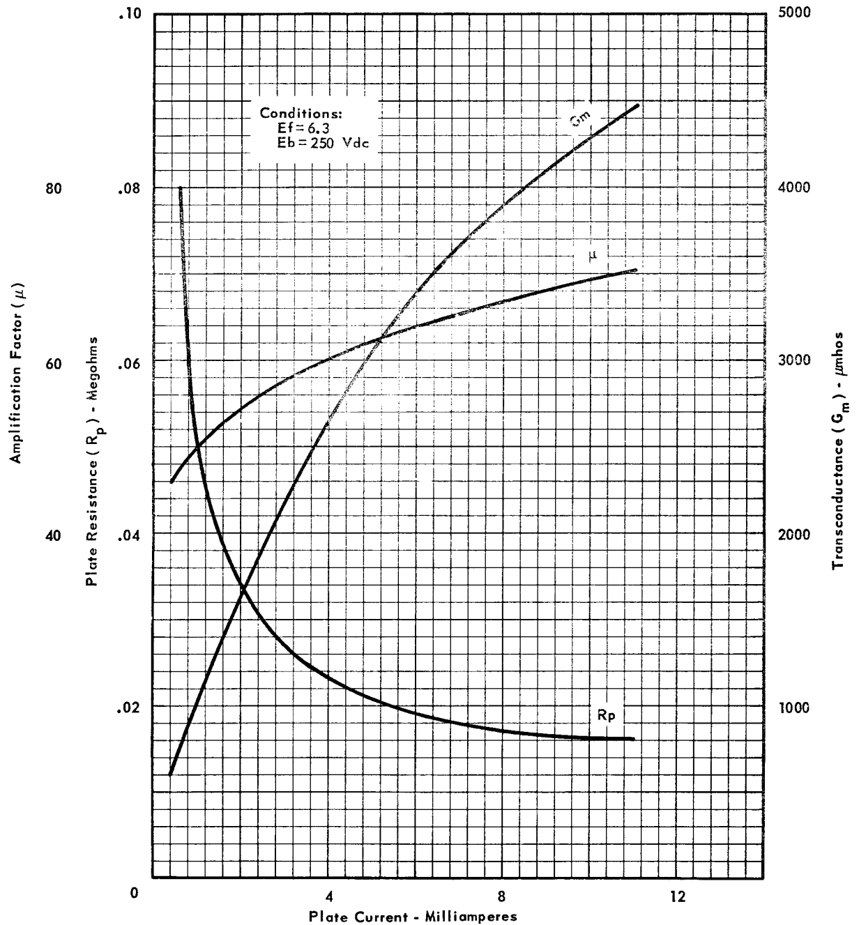
AVERAGE CHARACTERISTICS
