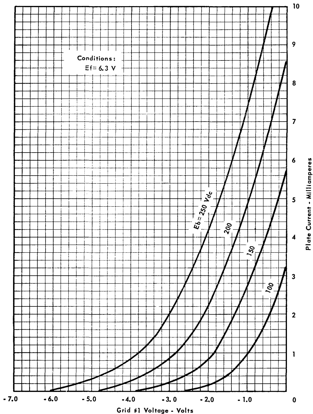
AVERAGE CHARACTERISTICS
