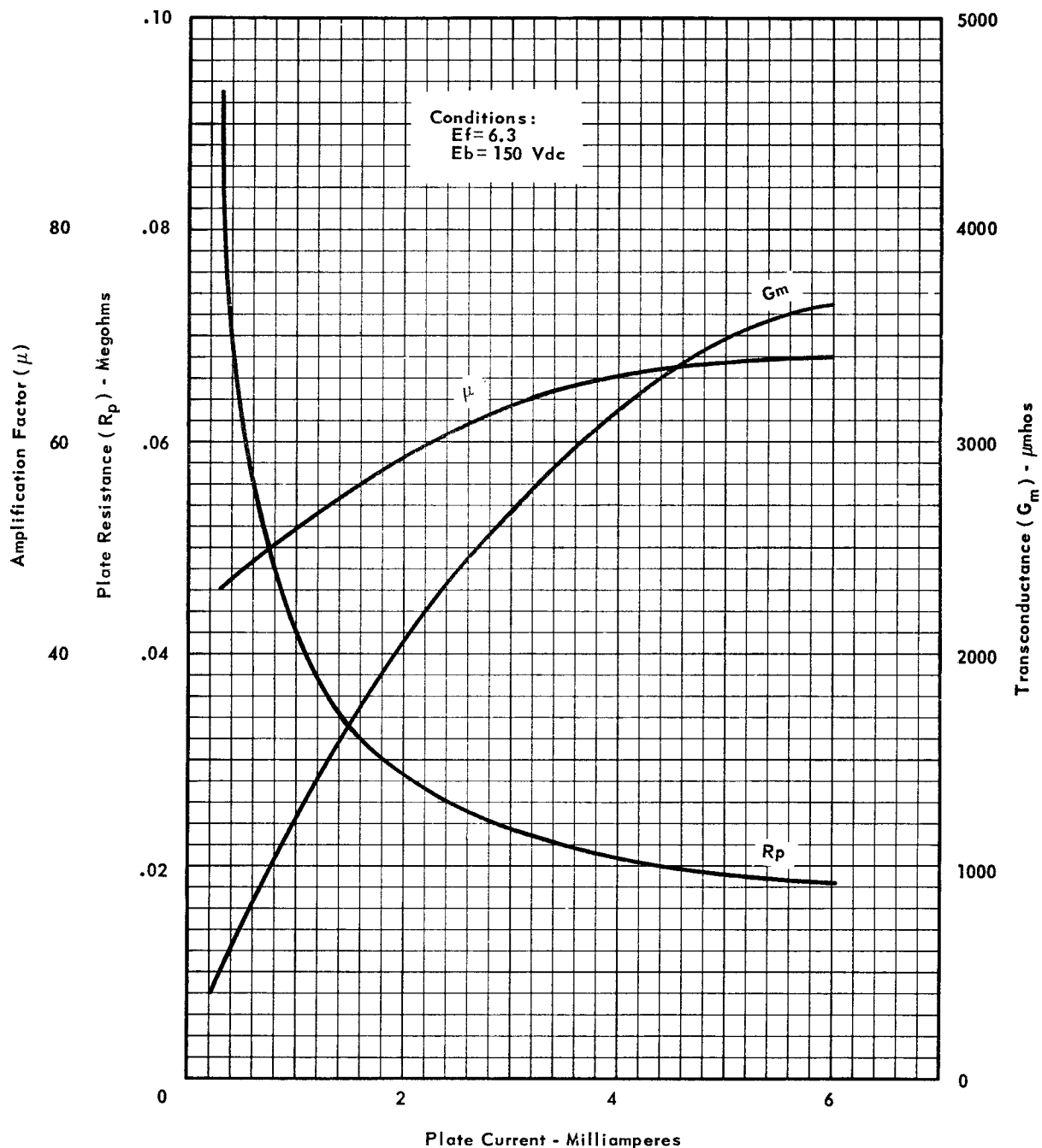
AVERAGE CHARACTERISTICS
