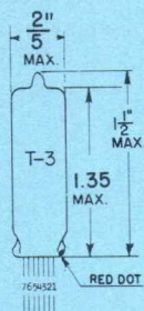
GLASS BULB
