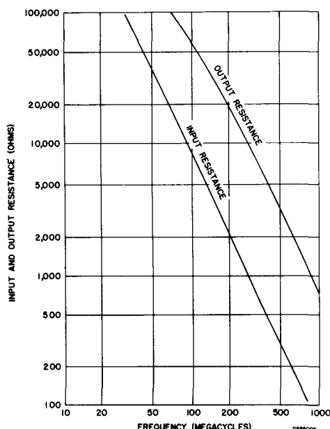
Figure 1—Input and output resistance vs frequency.
