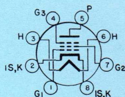
BOTTOM VIEW BASING DIAGRAM JEDEC 80C
