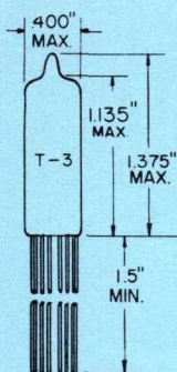
GLASS BULB SUBMINIATURE BUTTON FLEXIBLE LEADS BASE E8-10 OUTLINE DRAWING JEDEC 3-1
