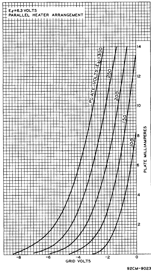
Fig. 4 - Average Characteristics for Each Unit of Type 6201.
