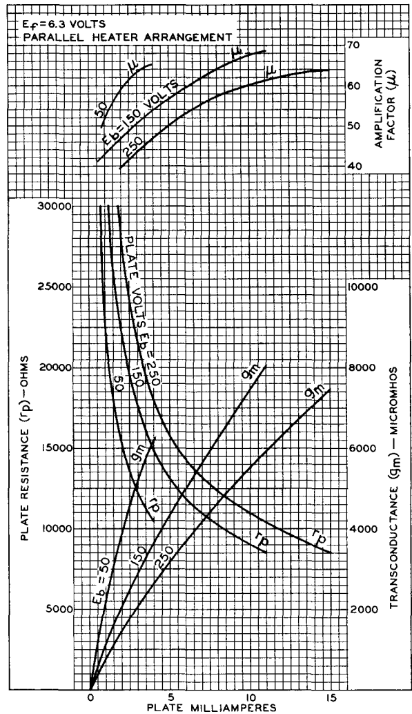
Fig. 2 - Average Characteristics for Each Unit of Type 6201.
