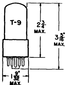
T-9 GLASS BULB INTERMEDIATE SHELL 8 PIN OCTAL LOW LOSS 88-6 OUTLINE DRAWING JEDEC 9-21
