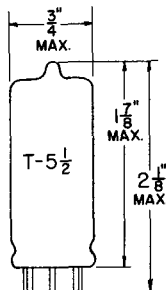
GLASS BULB
