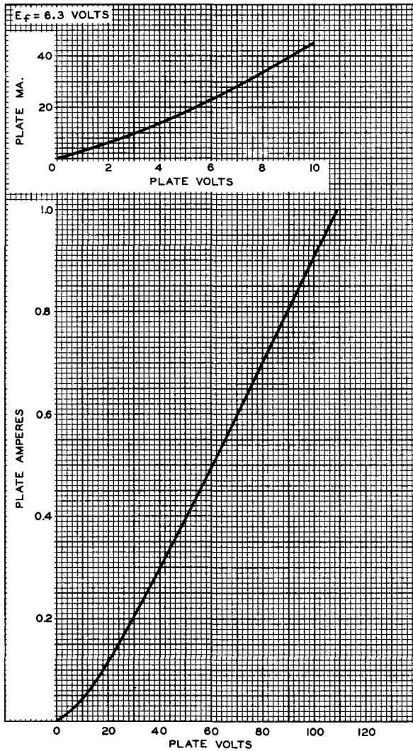
Fig. 1 - Average Plate Characteristics of Type 6173.
