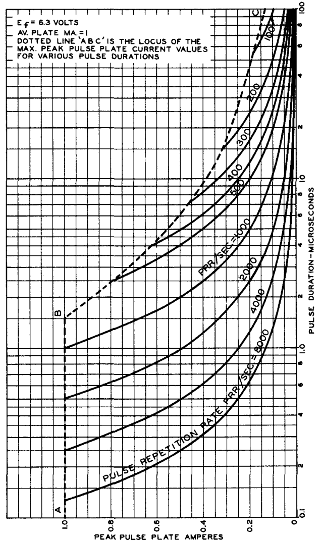
Fig. 2 - Pulse Rating Chart of Type 6173.
