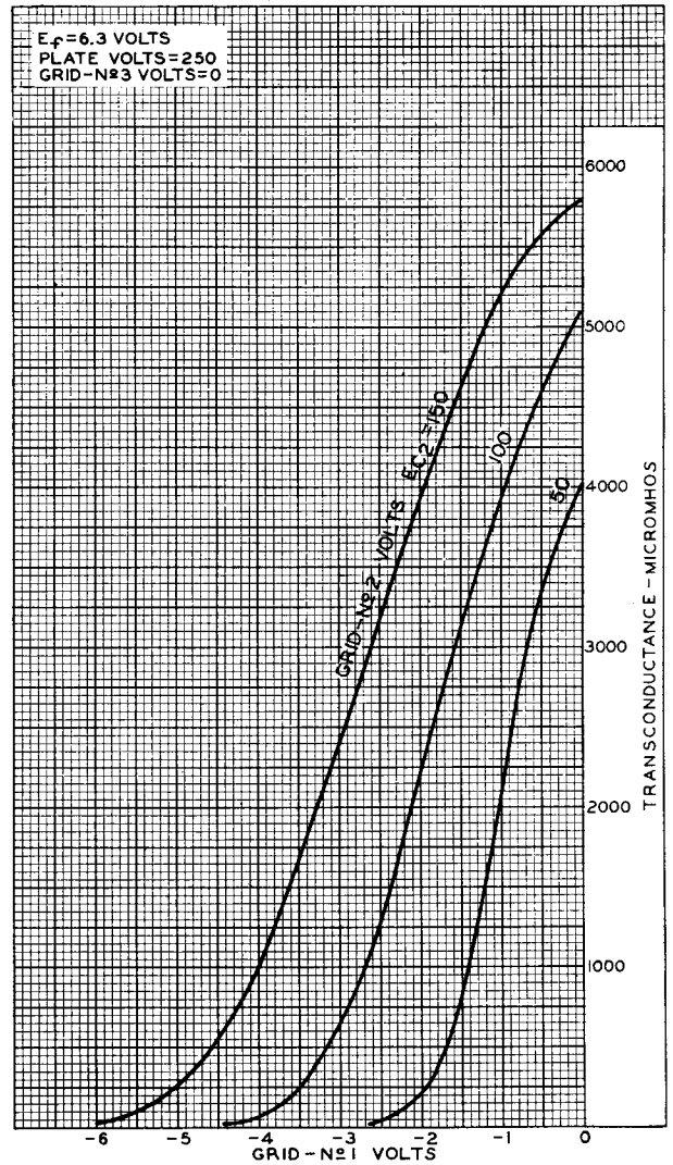
Fig.4 - Average Characteristics for Each Unit of Type 6136.
