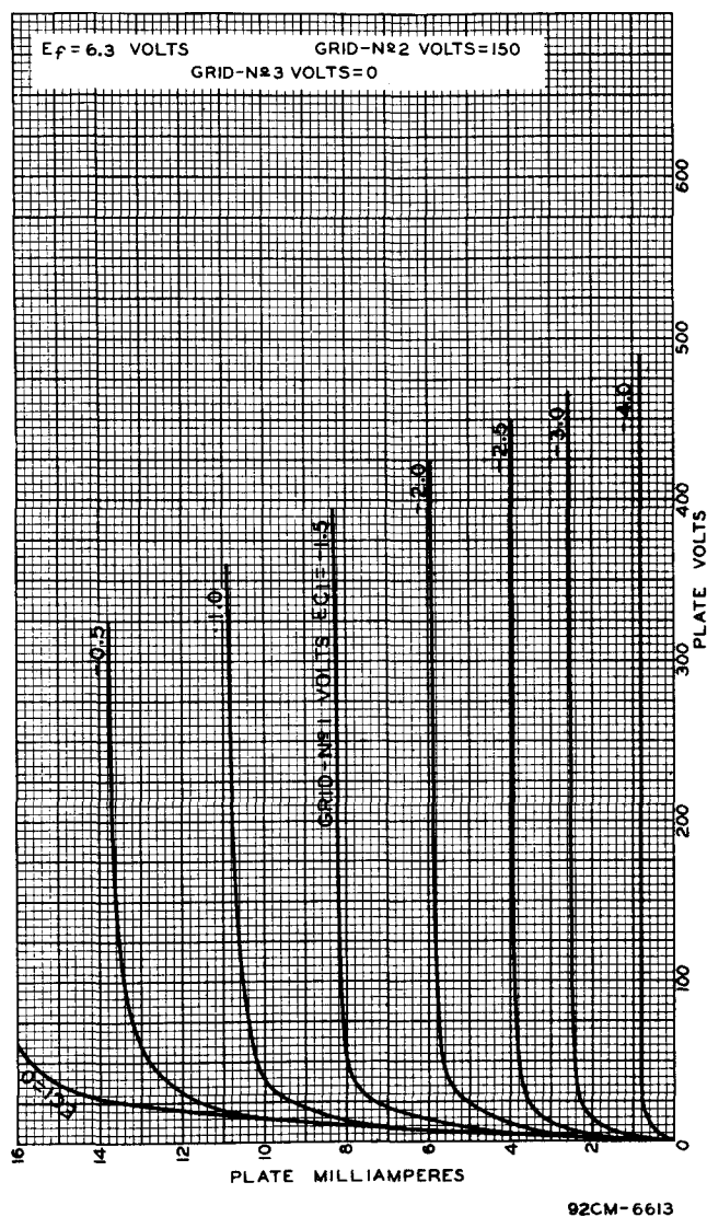
Fig. 2 - Average Characteristics for Each Unit of Type 6136.
