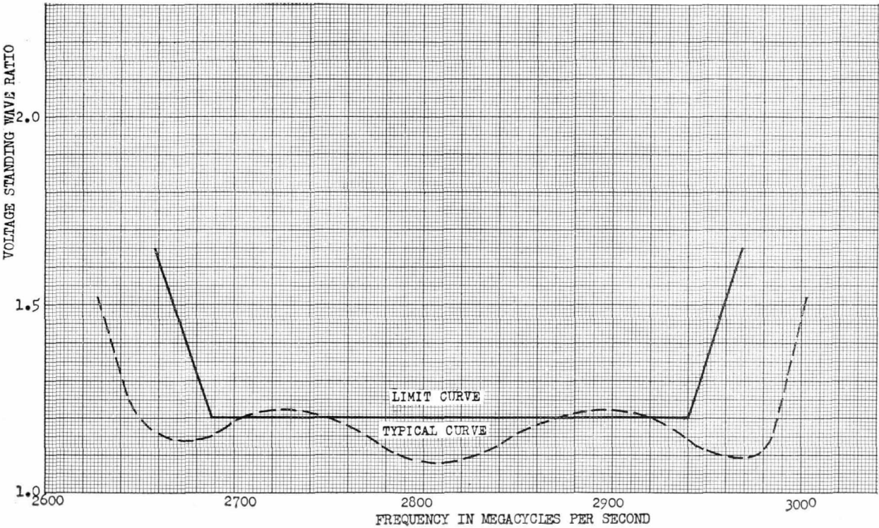
FREQUENCY-RESPONSE CURVE
