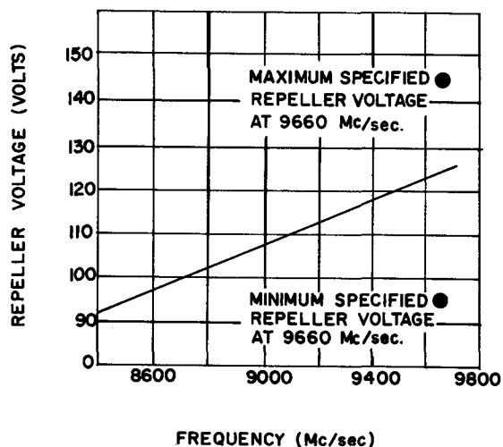
TYPICAL VARIATION OF REPELLER VOLTAGE V S FREQUENCY
