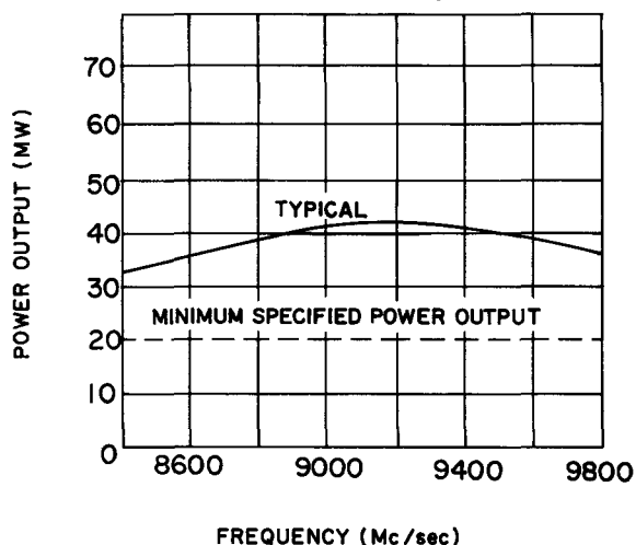
TYPICAL POWER OUTPUT V S FREQUENCY REPELLER VOLTAGE OPTIMIZED FOR EACH FREQUENCY
