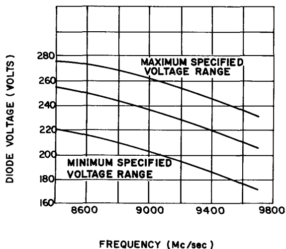
TYPICAL TUNER DIODE VOLTAGE V S FREQUENCY
