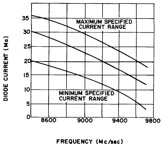
TYPICAL TUNER DIODE CURRENT V S FREQUENCY
