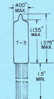
GLASS BULB SUBMINIATURE BUTTON 8 PIN BASE E8-10 0.17" TINNED FLEXIBLE LEADS OUTLINE DRAWING JEDEC 3-1
