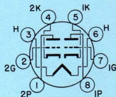
BOTTOM VIEW BASING DIAGRAM JEDEC 806
