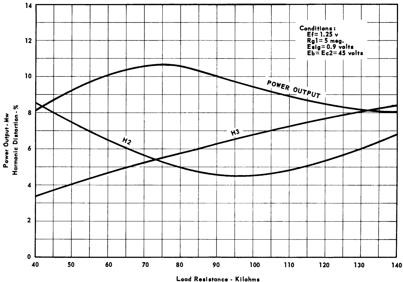
AVERAGE CHARACTERISTICS
