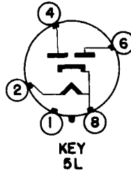
BASING DIAGRAM
