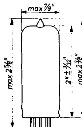
Tube outline
