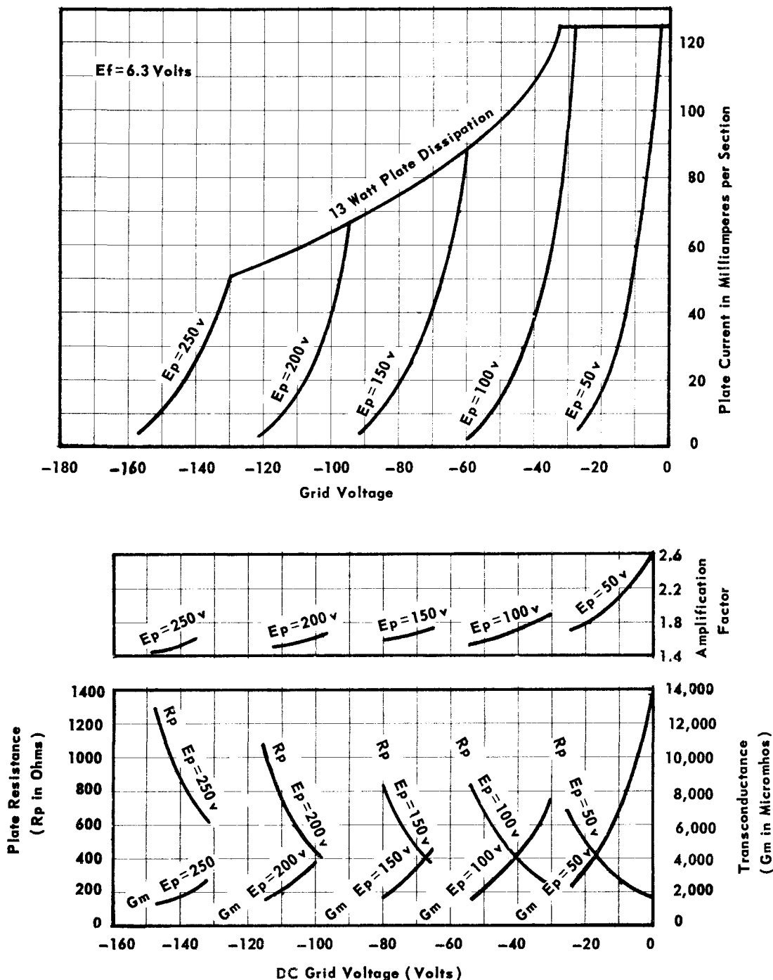
TRANSFER CHARACTERISTICS FOR EACH TRIODE SECTION
