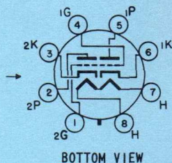
BOTTOM VIEW BASING DIAGRAM JEDEC 88D
