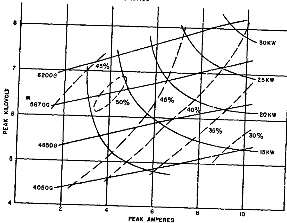
FIG. 2 TYPE 6027 OPERATING CHARACTERISTICS
