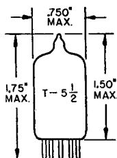
GLASS BULB MINIATURE BUTT 7 PIN E7-1
