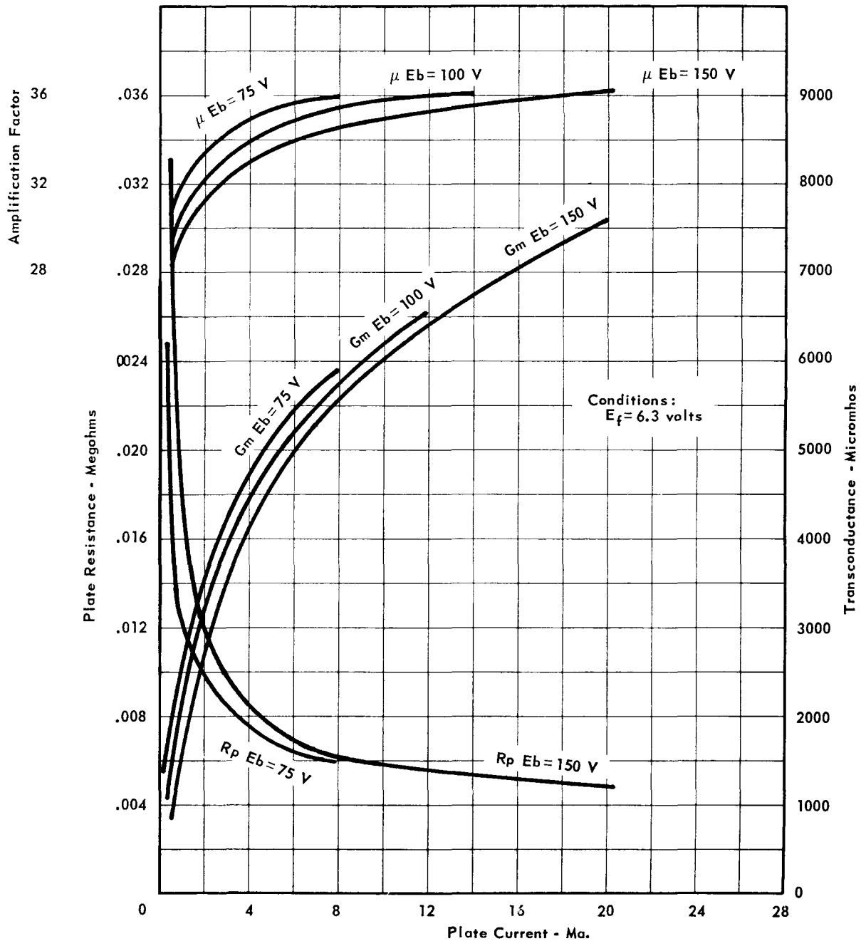
AVERAGE CHARACTERISTICS
