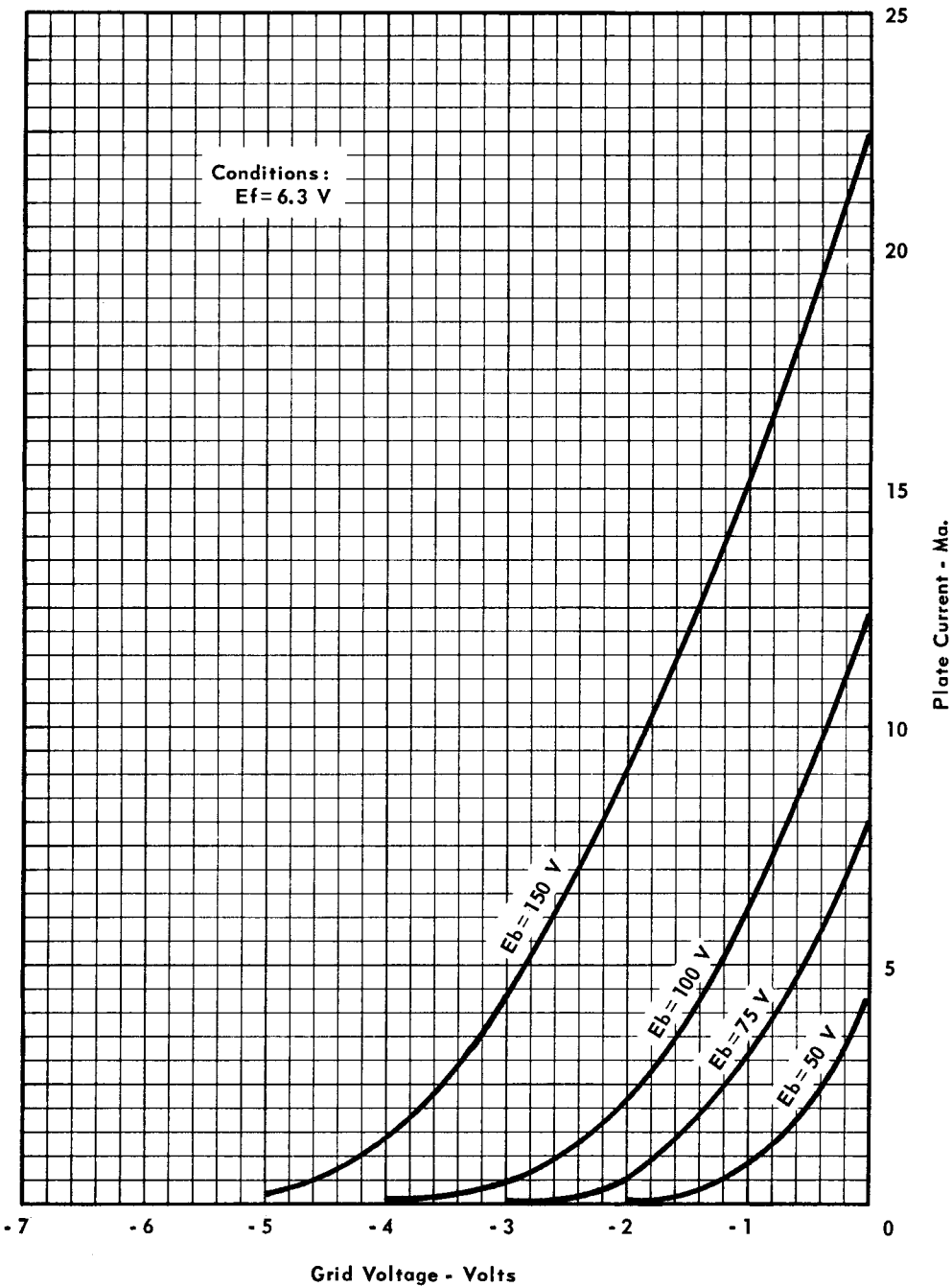
AVERAGE CHARACTERISTICS
