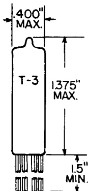
GLASS BULB
