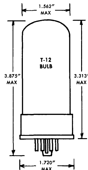
OUTLINE DRAWING
