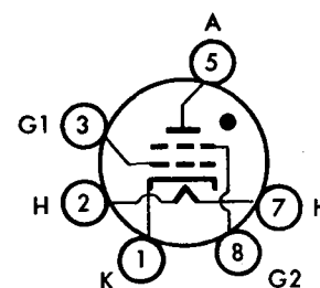
BASING DIAGRAM BOTTOM VIEW 6CO
