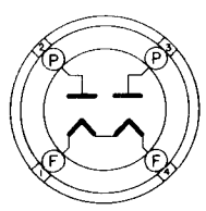
4C BOTTOM VIEW 5Z3
