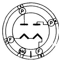
BOTTOM VIEW MEDIUM SHELL 5 PIN OCTAL
