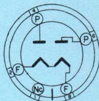
BOTTOM VIEW SPECIAL SKIRTED 5 PIN OCTAL
